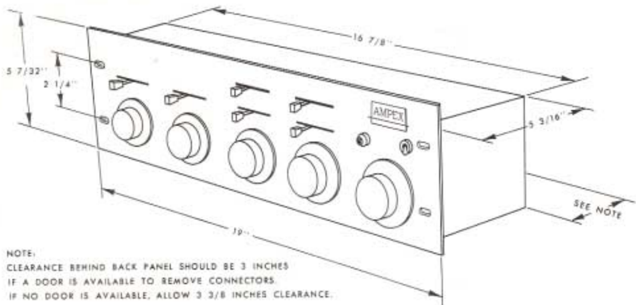
Mounting dimensions
